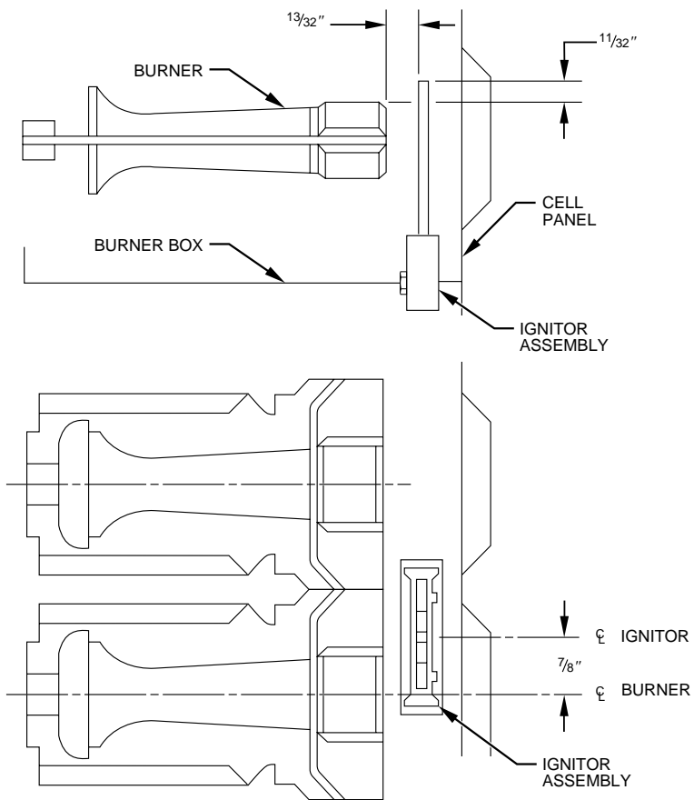
Fig. 31—Position of Igniter to Burner (Section 3)
