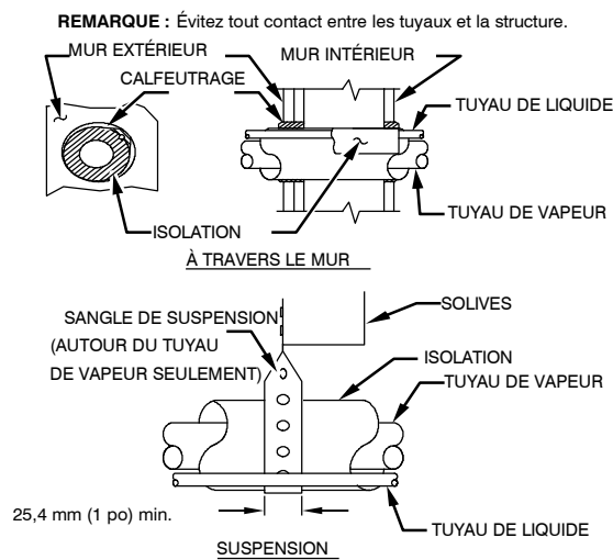
Figure 1 – Installation de la tuyauterie
