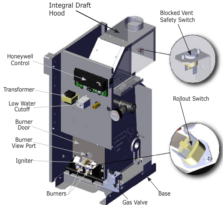
FIGURE 2 - BOILER FLUE GAS PASSAGEWAYS
