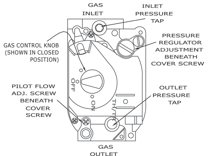
FIGURE 1- 1 - GAS VALVE
